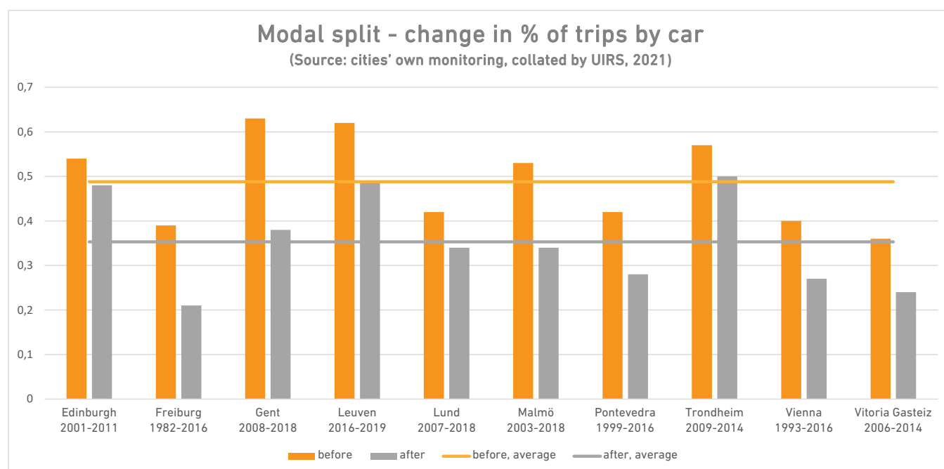
Figure 2.1: Modal Split
